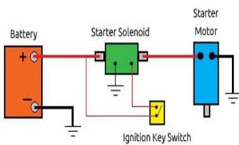
Solenoid Example Wiring Diagram
