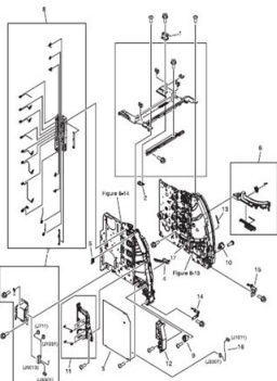
Figure 8-8. Internal components (1 of 4)
